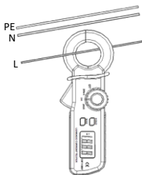
AC- Laststrom
